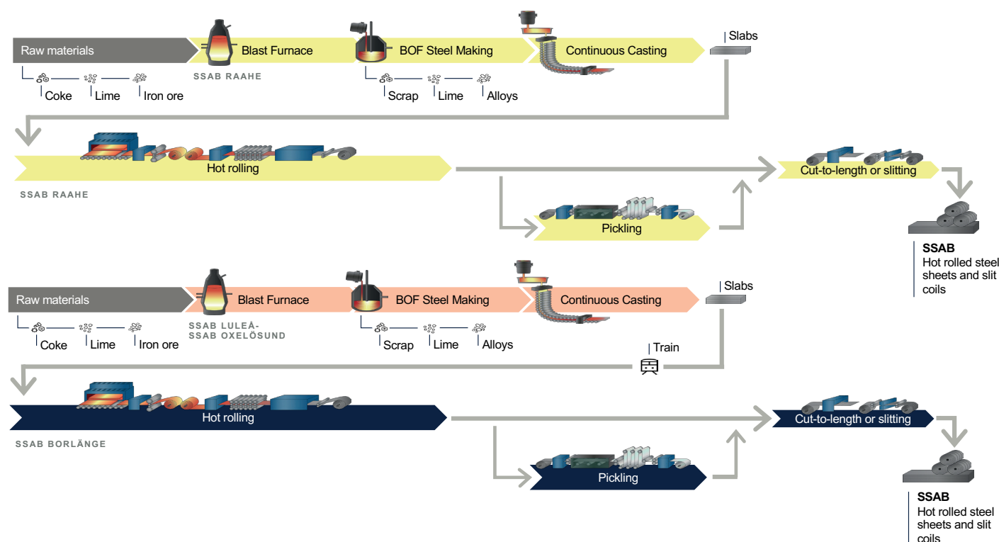
FIGURE 1. SSAB production sites and main process steps for blast furnace-based hot rolled steel sheets and slit coils.
