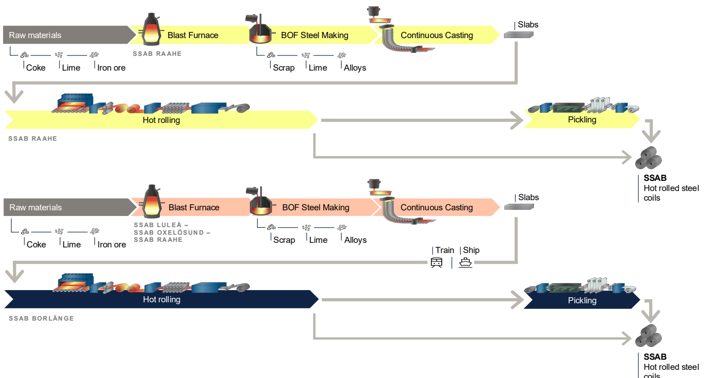
FIGURE 1. SSAB production sites and main process steps for the blast furnace-based hot rolled steel coils.
