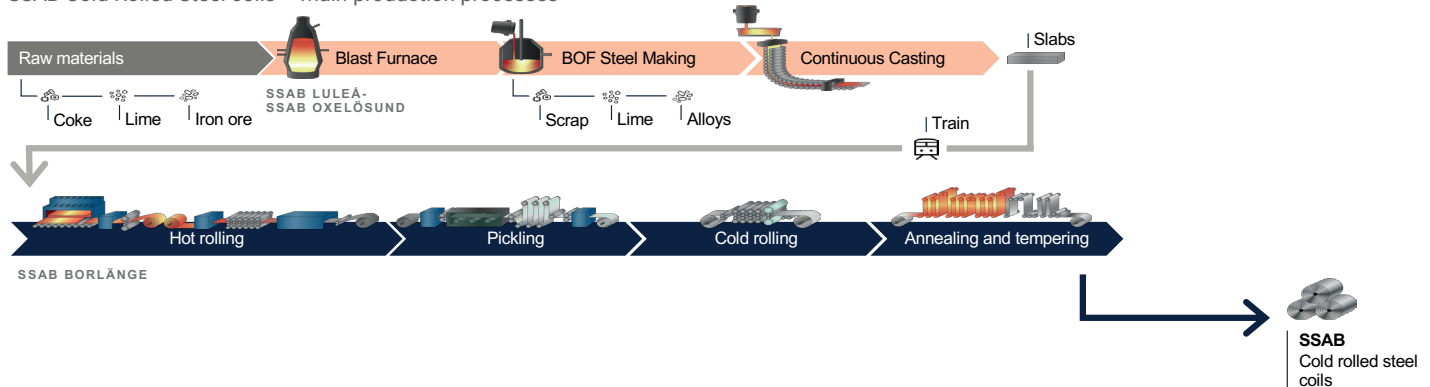
FIGURE 1. SSAB main production sites and process steps for blast furnace-based cold rolled steel coils.
