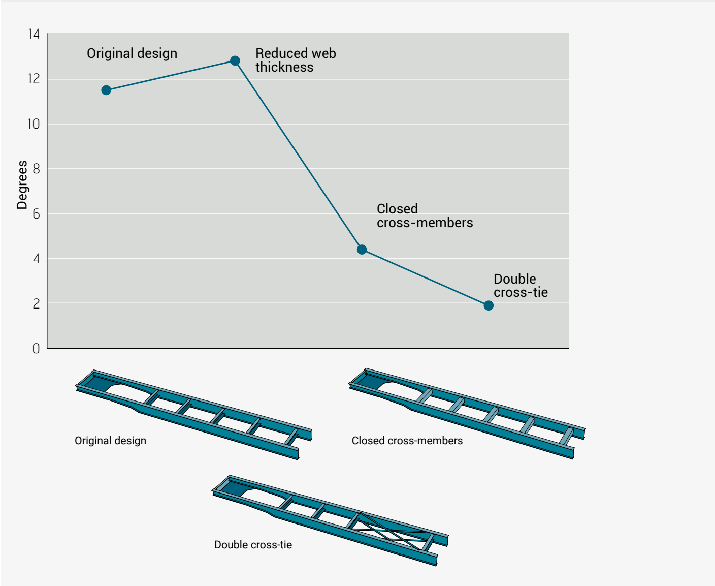
FIGURE 6 Comparison of the torsional resistance of a trailer chassis with open section cross-members to solutions with closed cross-member profiles and cross-bars.
