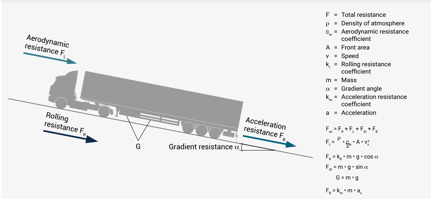
FIGURE 2 Overview of resistance factors affecting the fuel consumption of any road vehicle.
