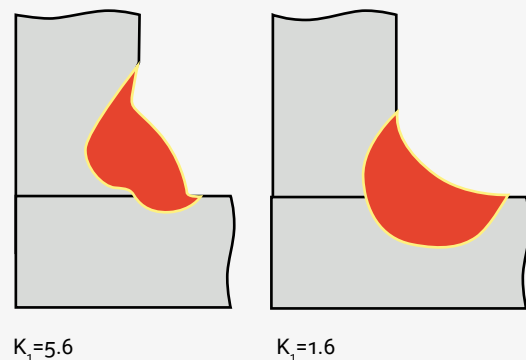
FIGURE 8 Sharp and smooth weld toe geometry.
