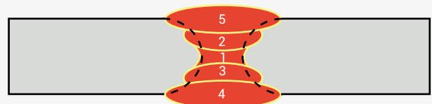
FIGURE 22 Use a symmetrical welding sequence.
